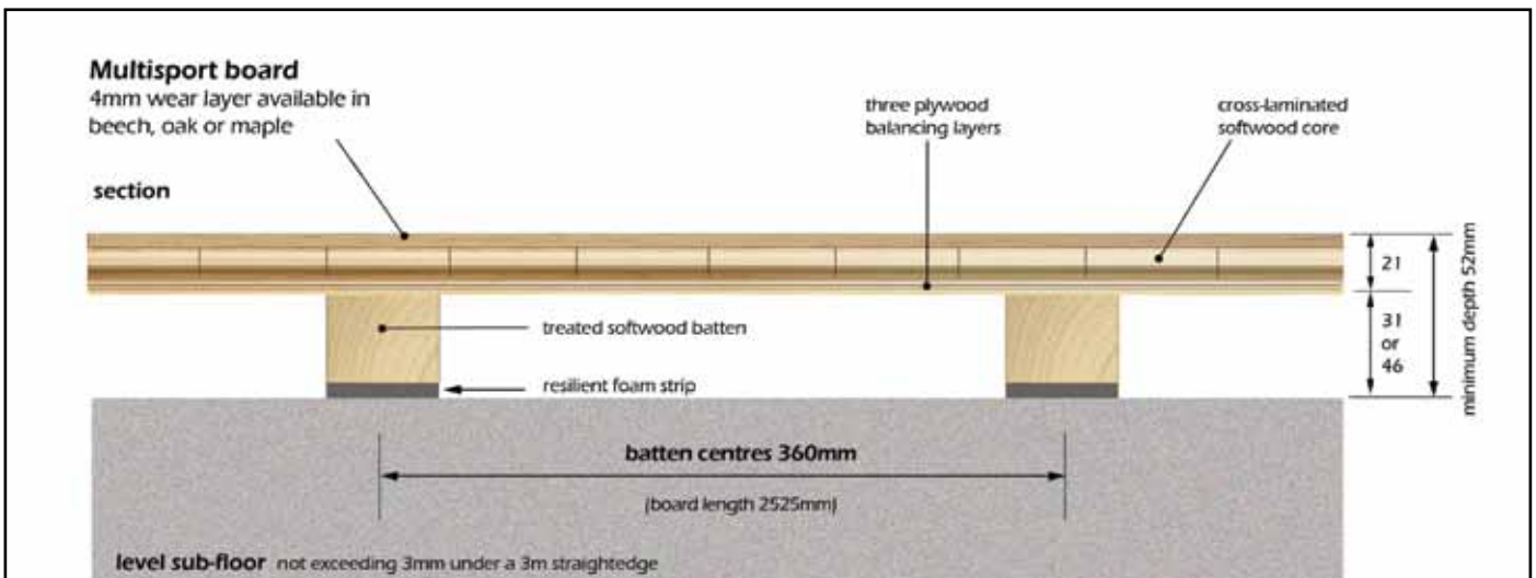
Reflex Sportsbat Batten System
