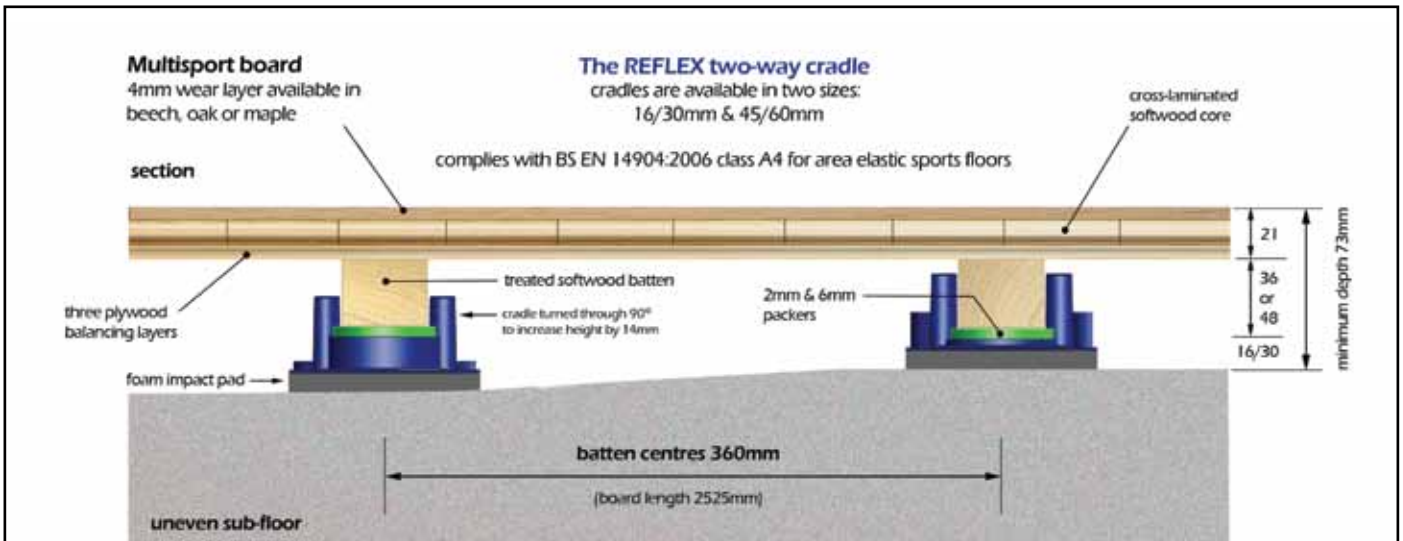
Reflex Levelling Cradle System
